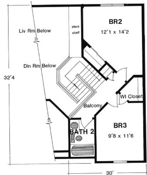
SECOND FLOOR 468 SF
