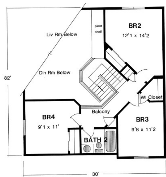
THE HUNTINGTON (4BR) 1509 SF
