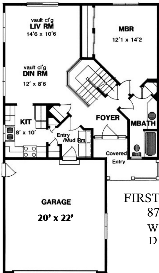
THE HUNTINGTON (4BR) 1509 SF
