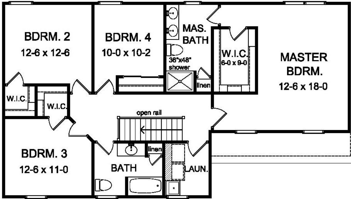
SECOND FLOOR 1213 SF
