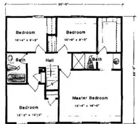
Second Floor Plan W/4 Bedrooms 840 SF
