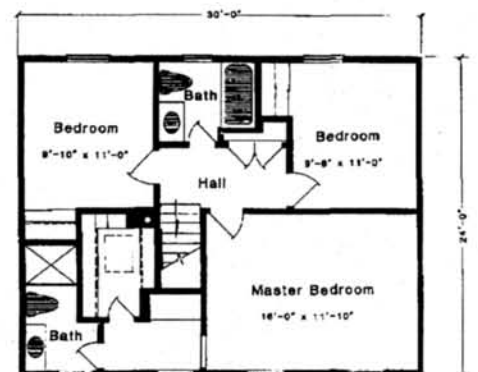
Second Floor Plan W/3 Bedrooms 720 SF
