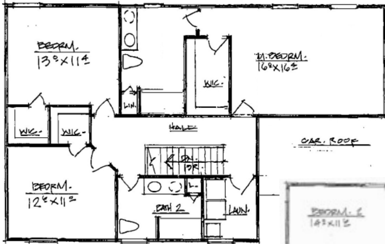
SECOND FLOOR 1033 SF (Std. MBath)
