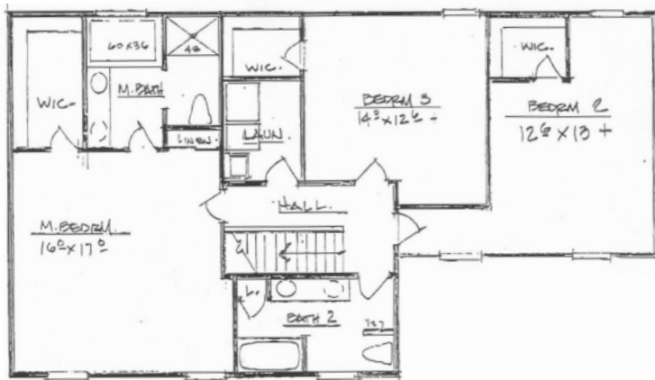
SECOND FLOOR 1214 SF (Upgraded Bath) Left
