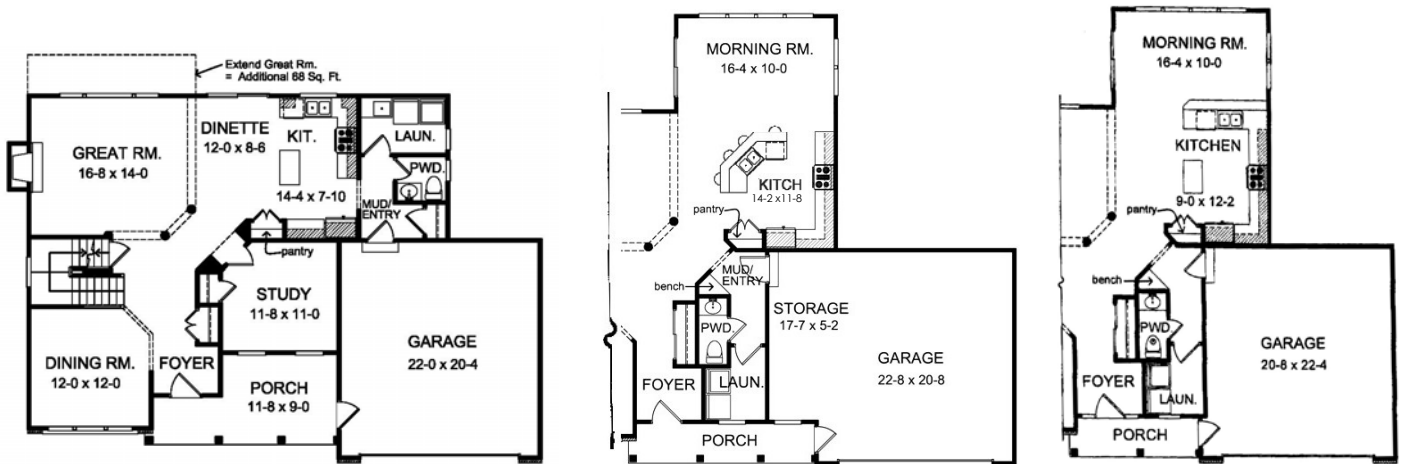
FIRST FLOOR A 1126 SF W- 52'-0" D- 37'-0"
